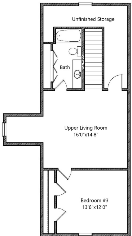
Upper Floor-748sf
