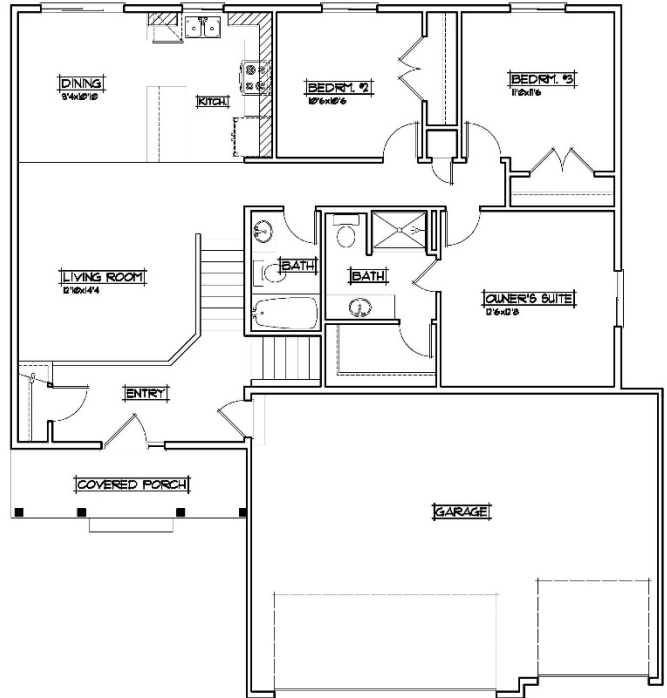
MAIN LEVEL FLOOR PLAN 061 80. FT. MAIN LEVEL
