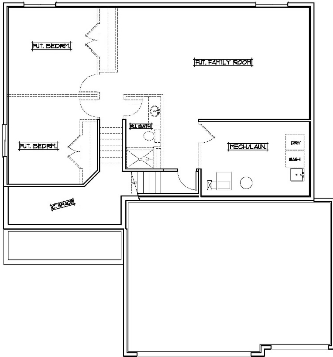
FOUNDATION PLAN
