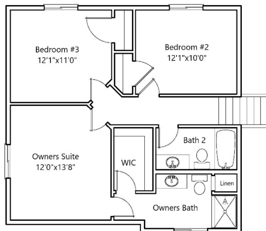
Upper Level-740sf
